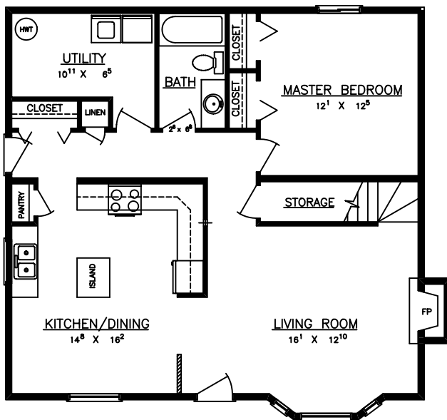
MAIN FLOOR
